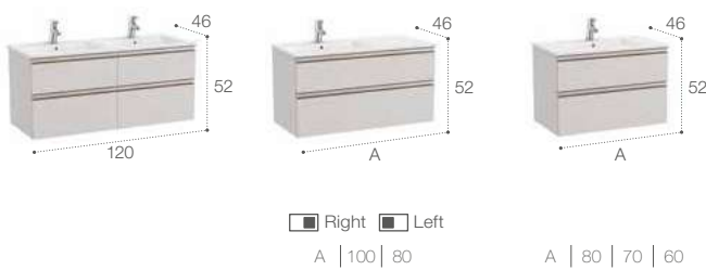
Unik compact (base unit and basin)
